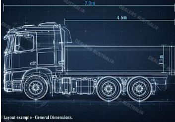
Layout example - General Dimensions.
